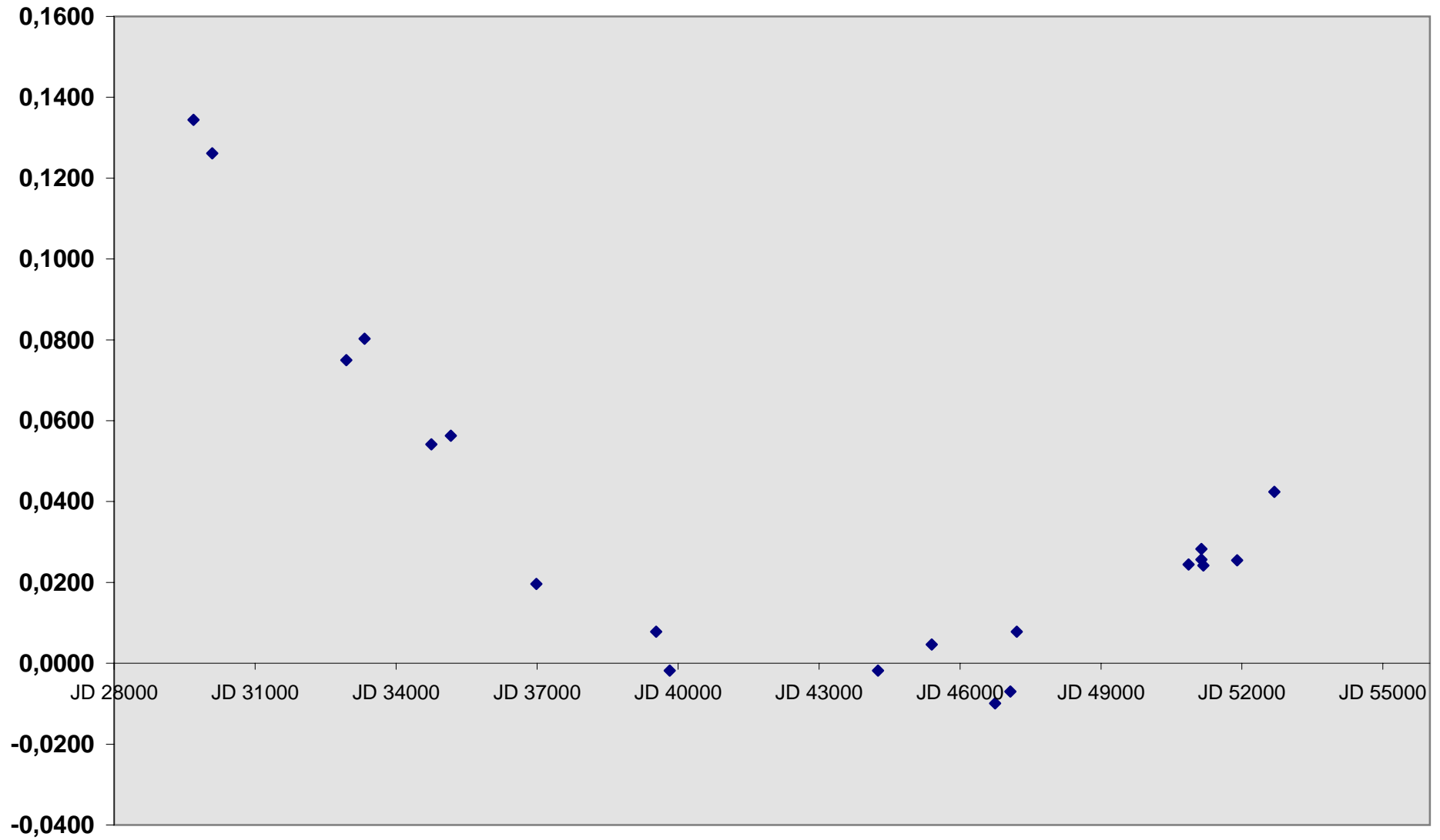
O-C diagram of V514 Mon (KL 1997)
